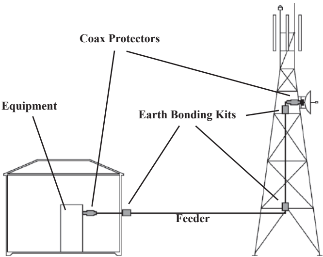
Figure 6: Typical Installation
