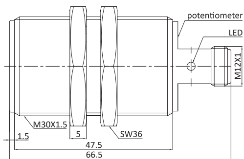
Fig. 3 Capacitive sensor with M12 connector (flush)
