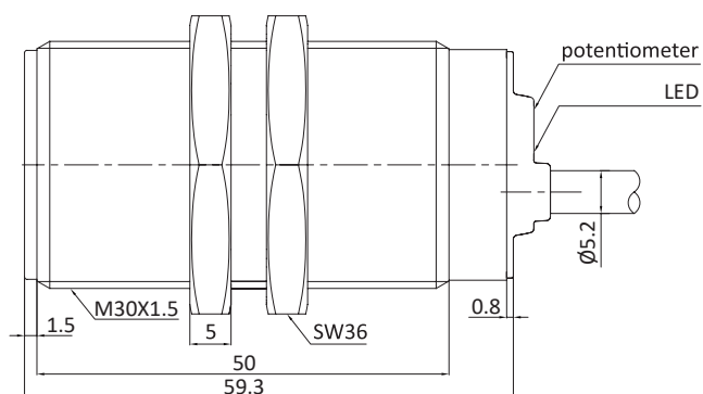
Fig. 1 Capacitive sensor with cable (flush)
