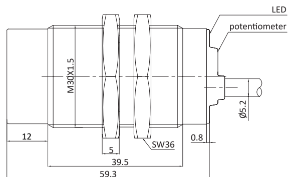
Fig. 2 Capacitive sensor with cable (non-flush)
