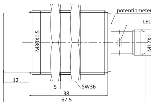
Fig. 4 Capacitive sensor with M12 connector (non-flush)
