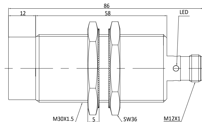
Fig. 4 Inductive sensor with M12 connector (non-flush)
