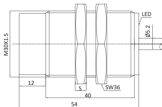
Fig. 1 Inductive sensor with cable (non-flush)
