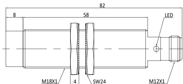
Fig. 4 Inductive sensor with M12 connector (non-flush)
