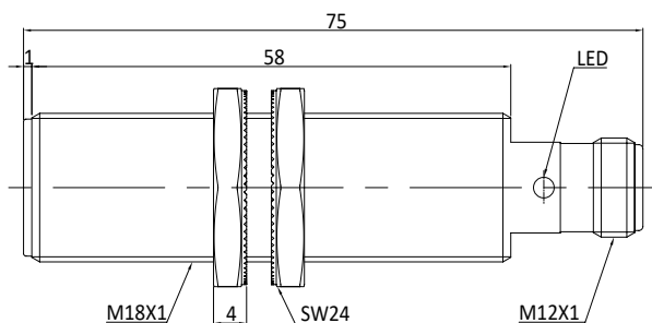
Fig. 3 Inductive sensor with M12 connector (flush)
