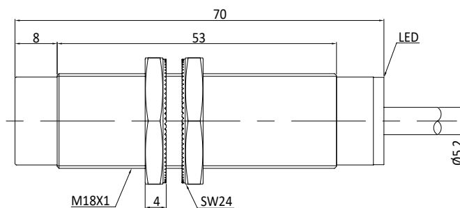
Fig. 2 Inductive sensor with cable (non-flush)
