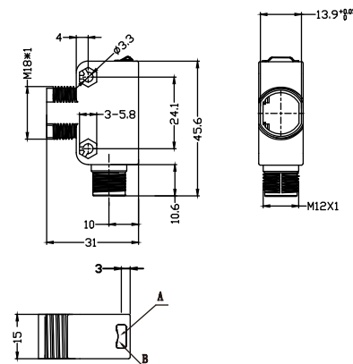
M12 Connector
