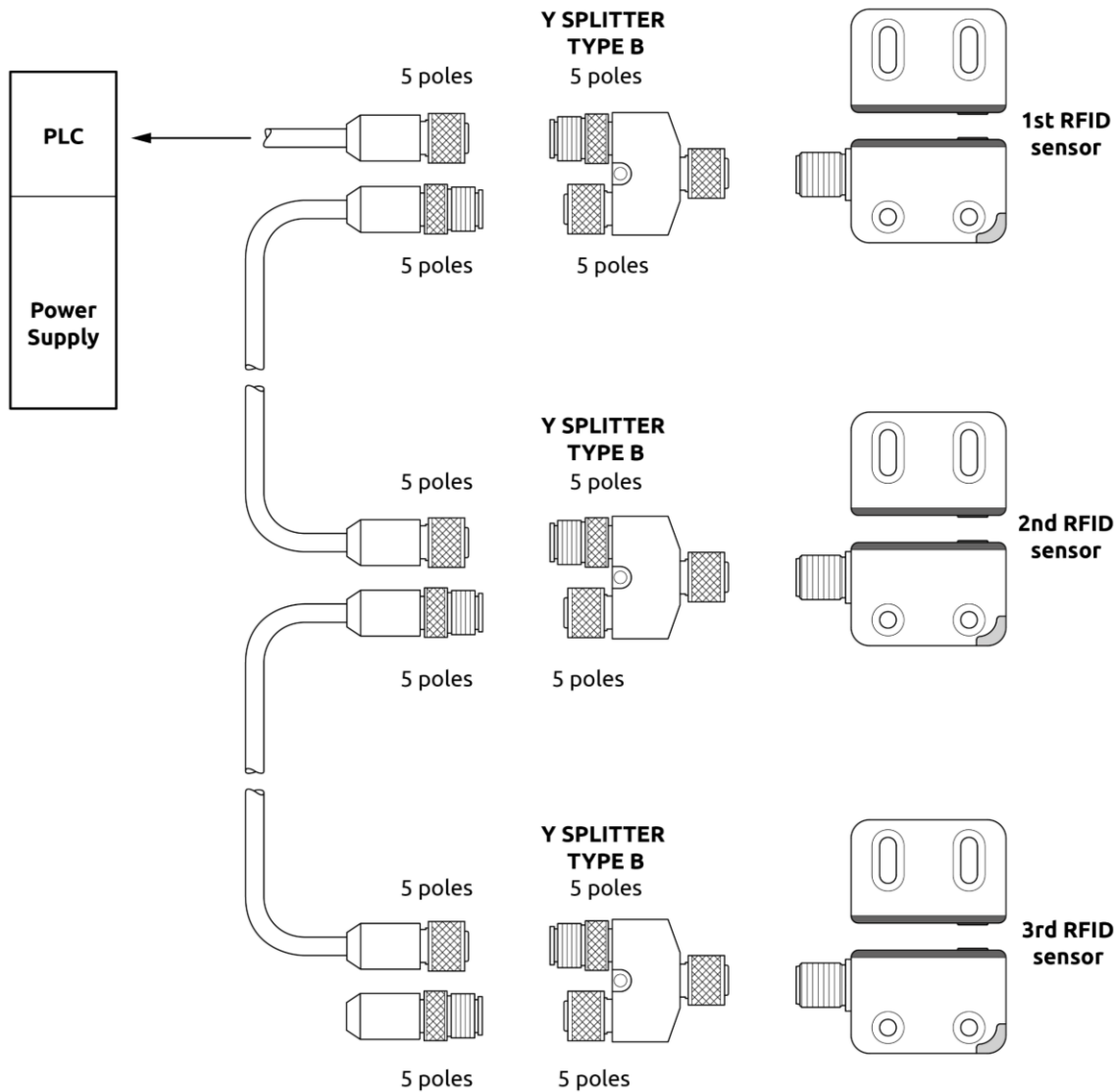
Figure 19 - Serial mode using "Splitter" connectors (R-Safe RFID Pro)
