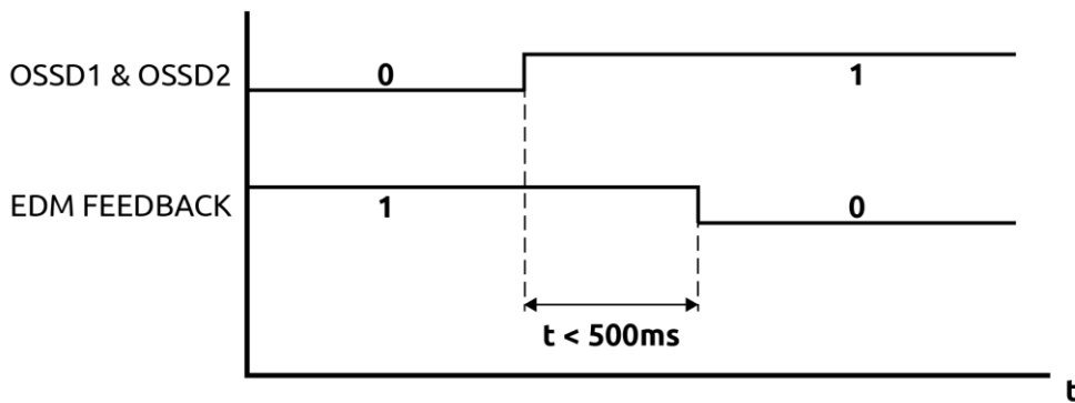
Figure 15 - Correct EDM timing
