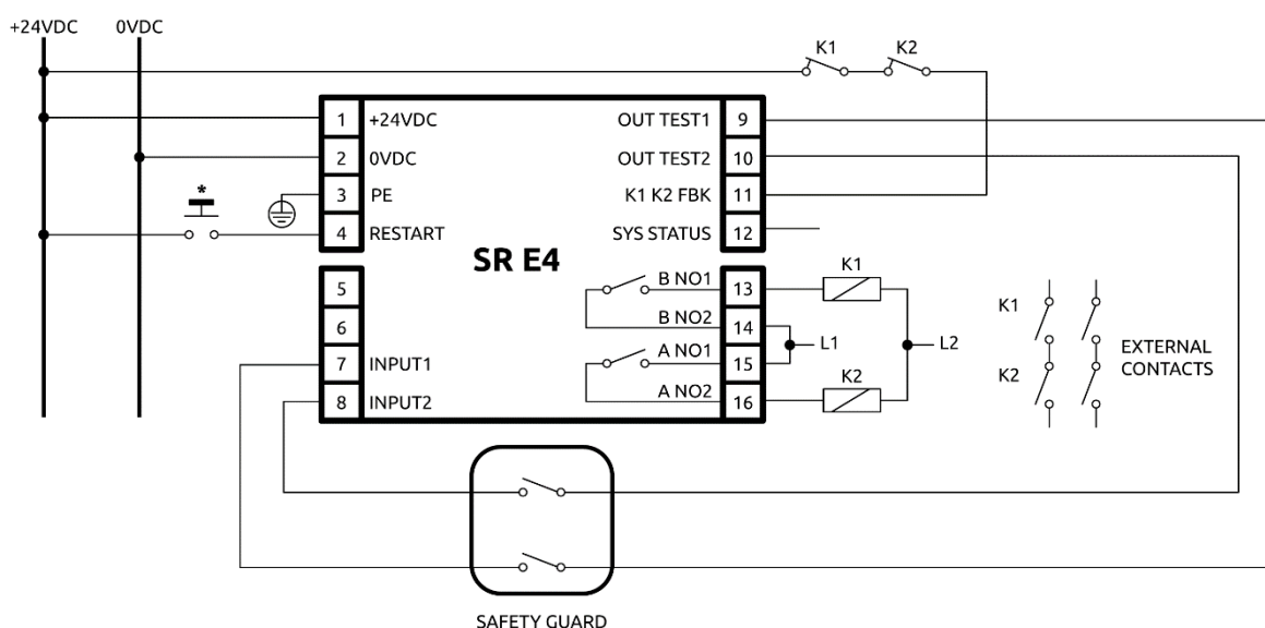
Figure 2 – Manual operation with K1 K2 relays
