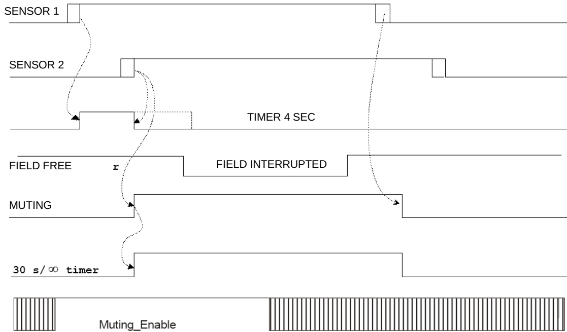
Figure 12 Muting cycle
