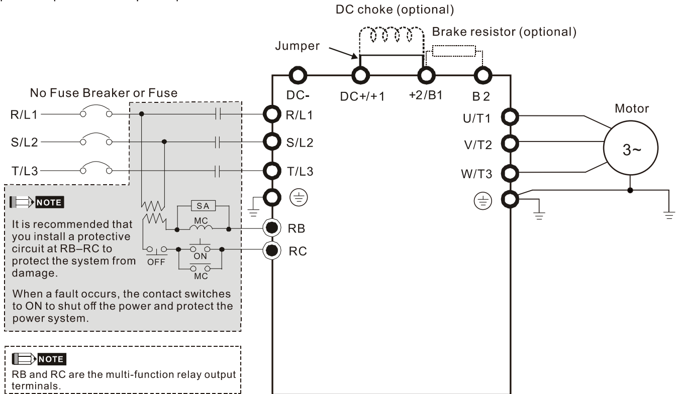
Wiring of DC reactor
