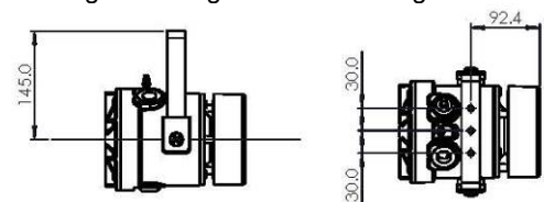
Fig. 1c Fixing Locations for Radial Horn
