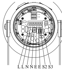
STExS1AC Terminals
