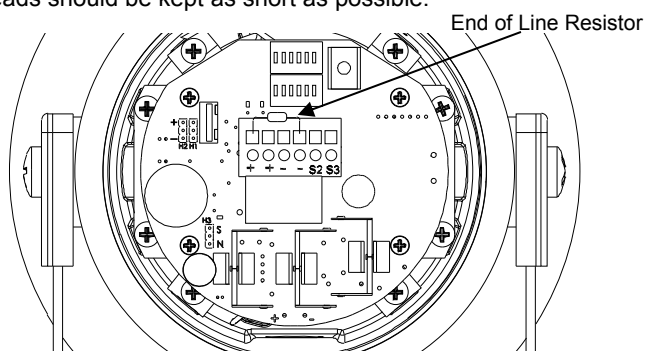
Fig. 8 End of Line Resistor Placement
