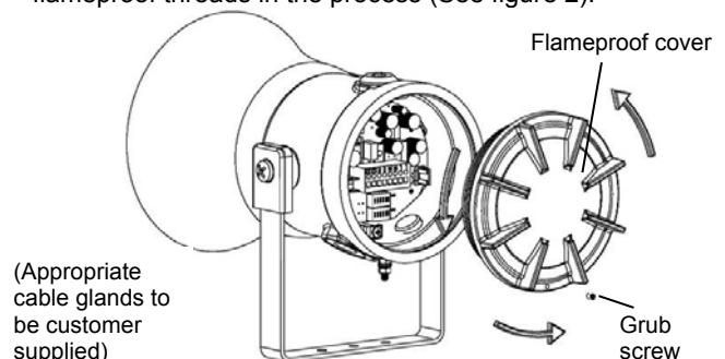
Fig. 2 Accessing the Explosion proof Enclosure.
