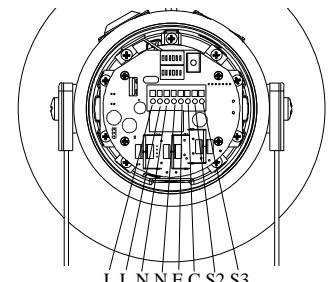
STExS2AC Terminals
