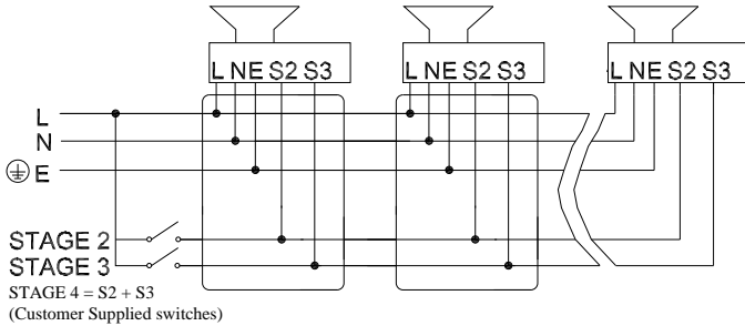
Fig 3a. STExS1AC Simplified Block Diagram
