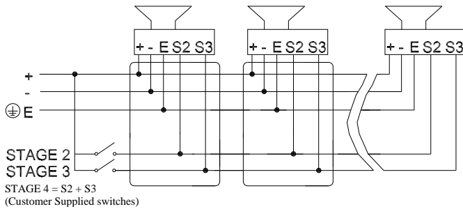
Fig. 5b DC Simplified Block Diagram (positive switching)
