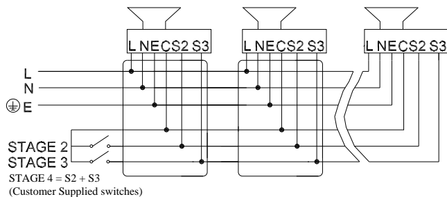
Fig 3b. STExS2AC Simplified Block Diagram
