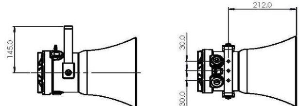
Fig 1b. Fixing Location for Large Horn
