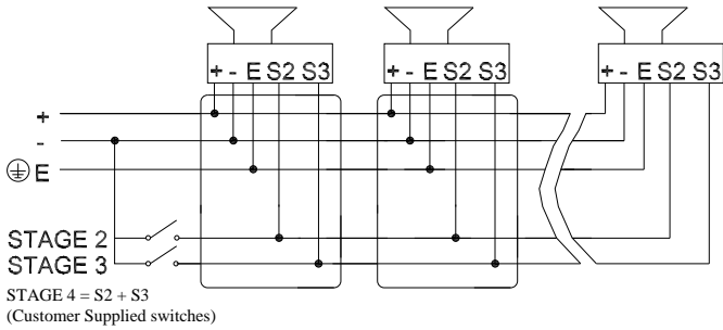
Fig. 5a DC Simplified Block Diagram (negative switching)
