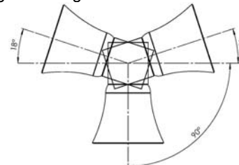
Fig. 1d Mounting Restrictions
