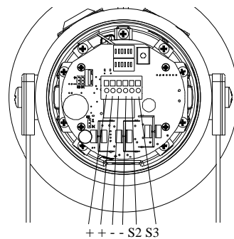
Fig. 6 DC Terminals
