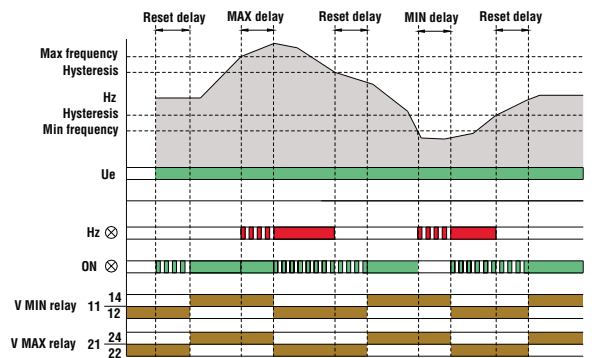
Maximum and minimum frequency (PMV80N)
