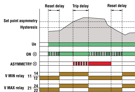
Asymmetry (PMV70N)
